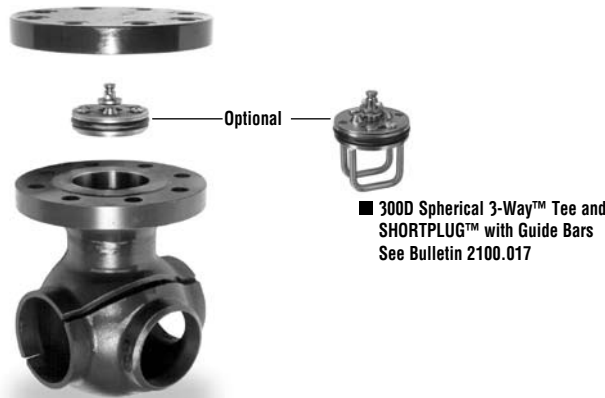
■ 300 D Spherical 3-WAY™ Tee See Bulletin 2100.008
