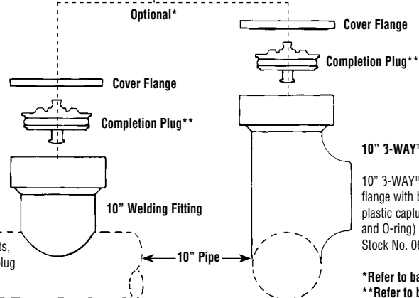
Valve-to-Fitting Adapter 06-5724-0012
